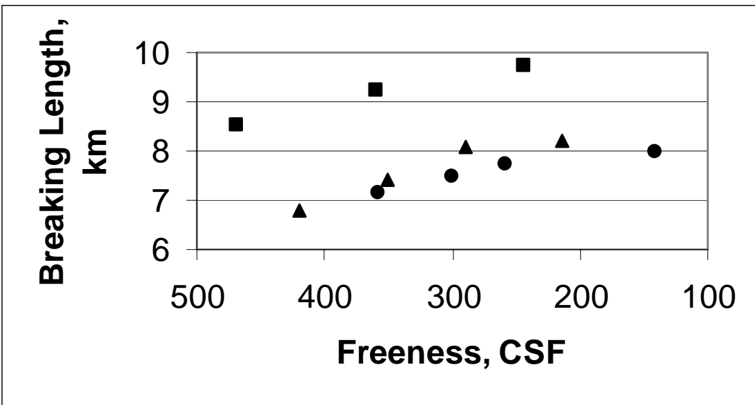
Figure 3. Tensile strength of bleached cotton stalk pulps versus southern hardwood ● = American cotton ▲ = Egyptian cotton ■ = hardwood
